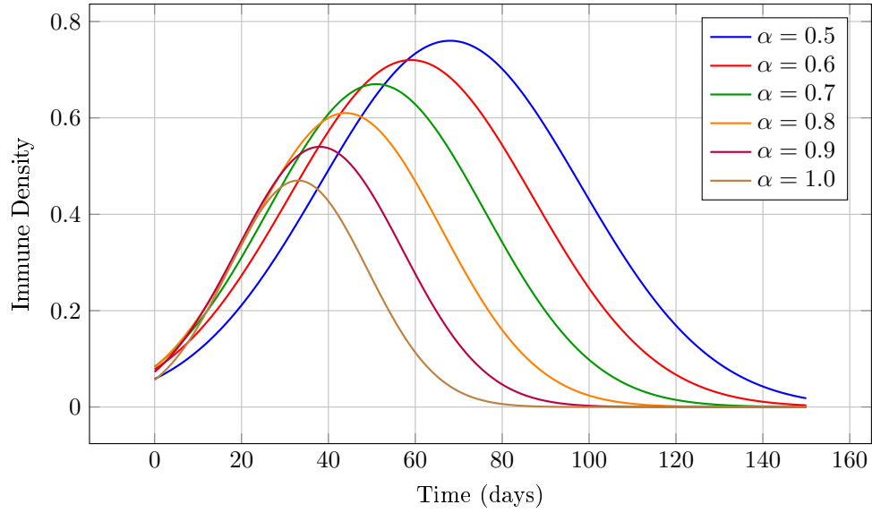
Figure 2: Numerical immune responses for different \alpha
