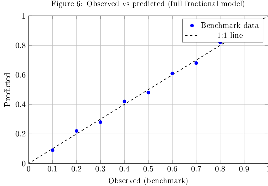
Figure 6: Observed vs predicted for the full fractional model. The R^2 ranges from 0.72 to 0.89.
