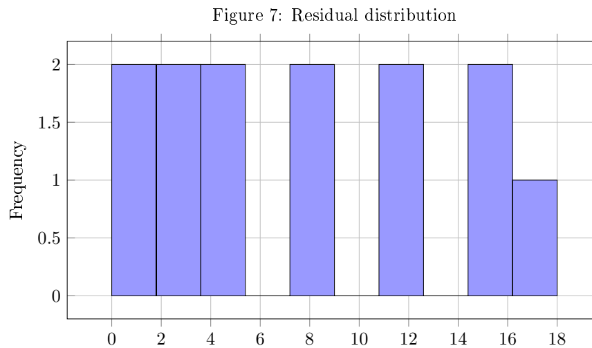
Figure 7: Histogram of residuals for the full fractional model, showing approximate normality.
