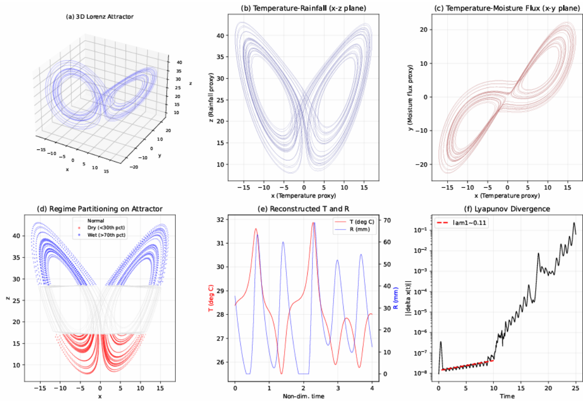
Figure 2: Lorenz attractor phase portraits and ASAL climate variable mapping. (a) 3D phase portrait on the Lorenz strange attractor. (b) x - z projection: temperature vs. rainfall proxies. (c) x - y projection: temperature vs. moisture flux. (d) Regime partitioning: dry (red, <30th percentile of z ), normal (gray), wet (blue, >70th percentile of z ) regimes on the attractor. (e) Reconstructed temperature and rainfall time series from Lorenz. (f) Divergence of nearby trajectories demonstrating the Lorenz butterfly effect ( \lambda_1 \approx 0.90 ).
