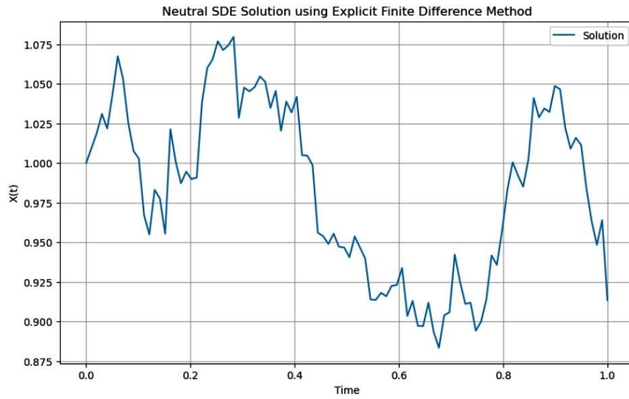
Figure 1. Neutral Stochastic Differential Equation solution using explicit finite difference Method
